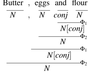
Figure 6: CCGbank analysis of coordination
