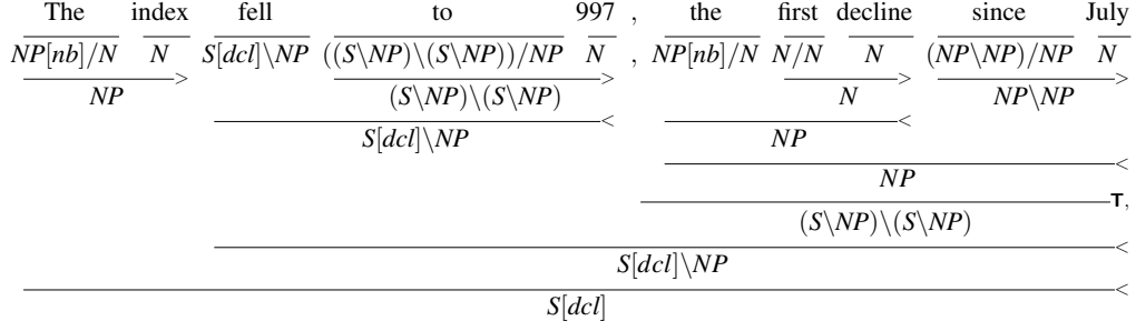
Figure 5: The type change rule , NP \rightarrow (S\backslash NP)\backslash (S\backslash NP) is applied in the fifth row
