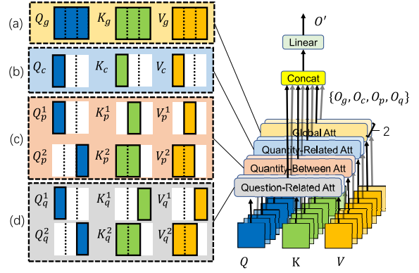
Figure 3: Group attention: (a) Global attention; (b) Quantity-related attention; (c) Quantity-pair attention; (d) Question-related attention.
