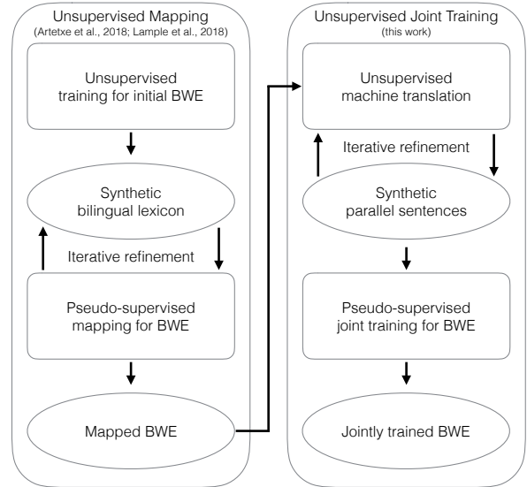
Figure 1: Our joint training framework is on top of existing unsupervised mapping methods.
