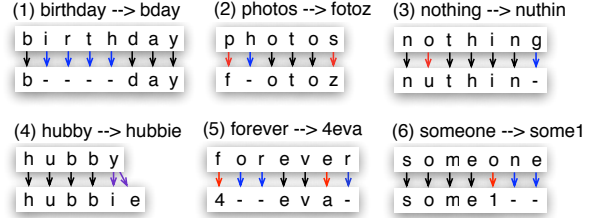
Figure 1: Examples of nonstandard tokens generated by performing letter transformation on the dictionary words.
