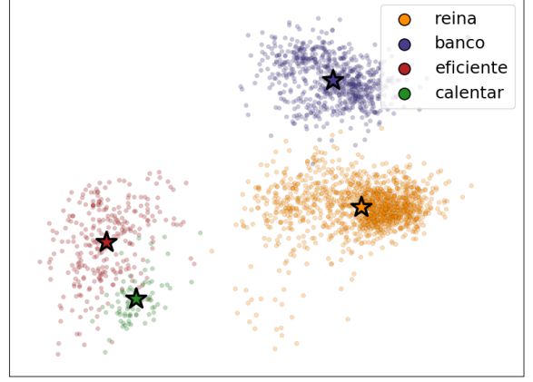
Figure 1: A two dimensional PCA showing examples of contextual representations for four Spanish words. Their corresponding anchors are presented as a star in the same color. (best viewed in color)
