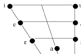
Figure 1: Bāsàá vowels (Makasso and Lee, 2015)
