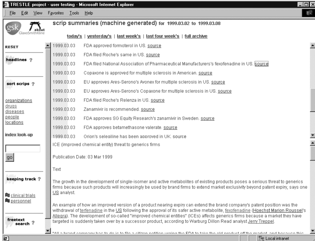
Figure 3: TRESTLE Interface: SCAT
