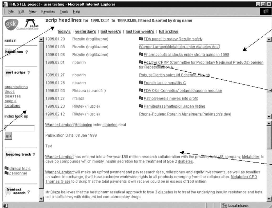
Figure 2: TRESTLE Interface: NEAT
