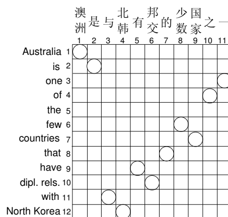
Figure 1: An aligned Chinese-English sentence pair.
