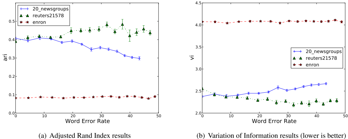
Figure 5: Results for the clustering experiments on the three synthetic OCR datasets with TNPD feature selection.
