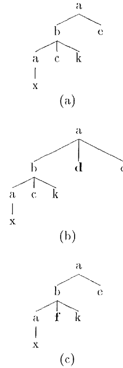
Figure 2: Structural and leaf label differences between trees.
