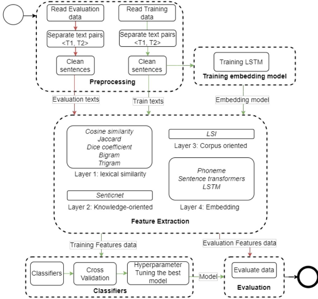
Figure 1: System General Pipeline
