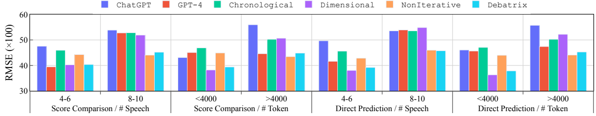
Figure 5: Winner prediction RMSE on DebateArt debates with different numbers of speeches (left) or tokens (right). Note that Debatrix (light blue bar) always reaches a relatively low RMSE regardless of the number of speeches or tokens; no other model can achieve this.
