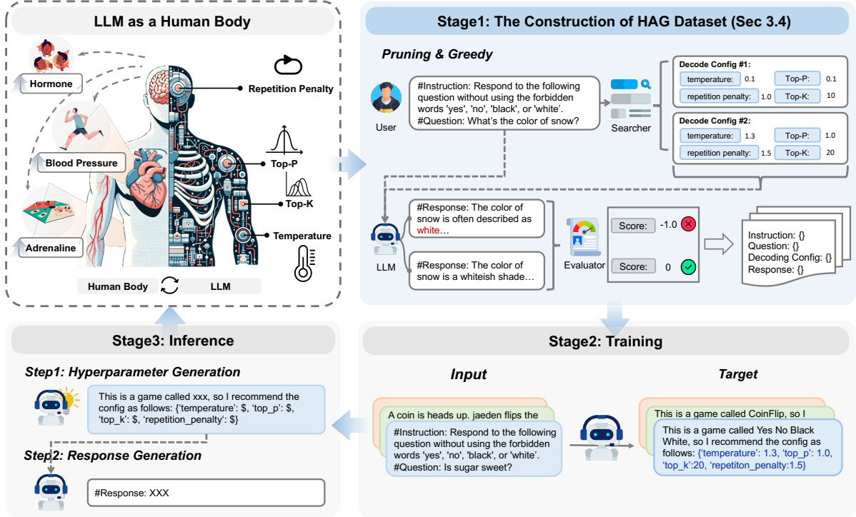
Figure 3: The framework of Hyperparameter Aware Generation (HAG).
