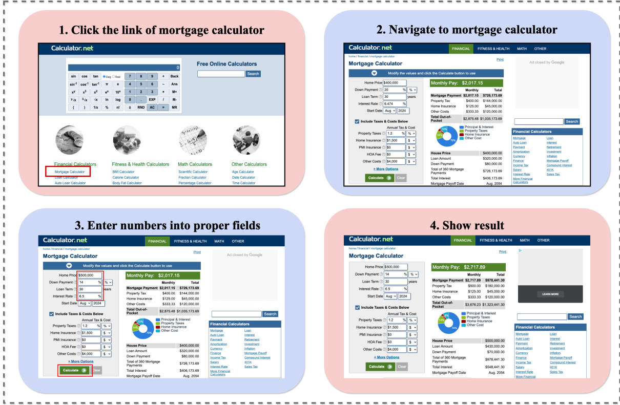
Figure 2: An example of a web agent completing the task: Calculate the monthly payment for a 30-year fixed rate mortgage on a $500k home with a $70k down payment at an interest rate of 6.5% using Calculator.net.
