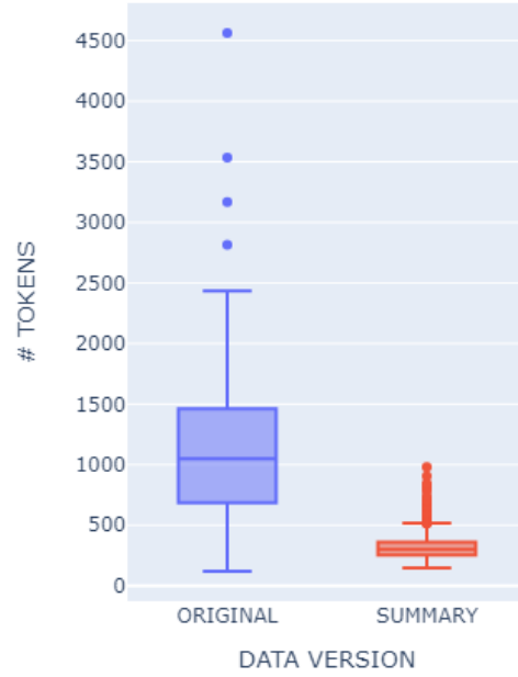
Figure 3: Distribution of Llama tokens for the EHR data.
