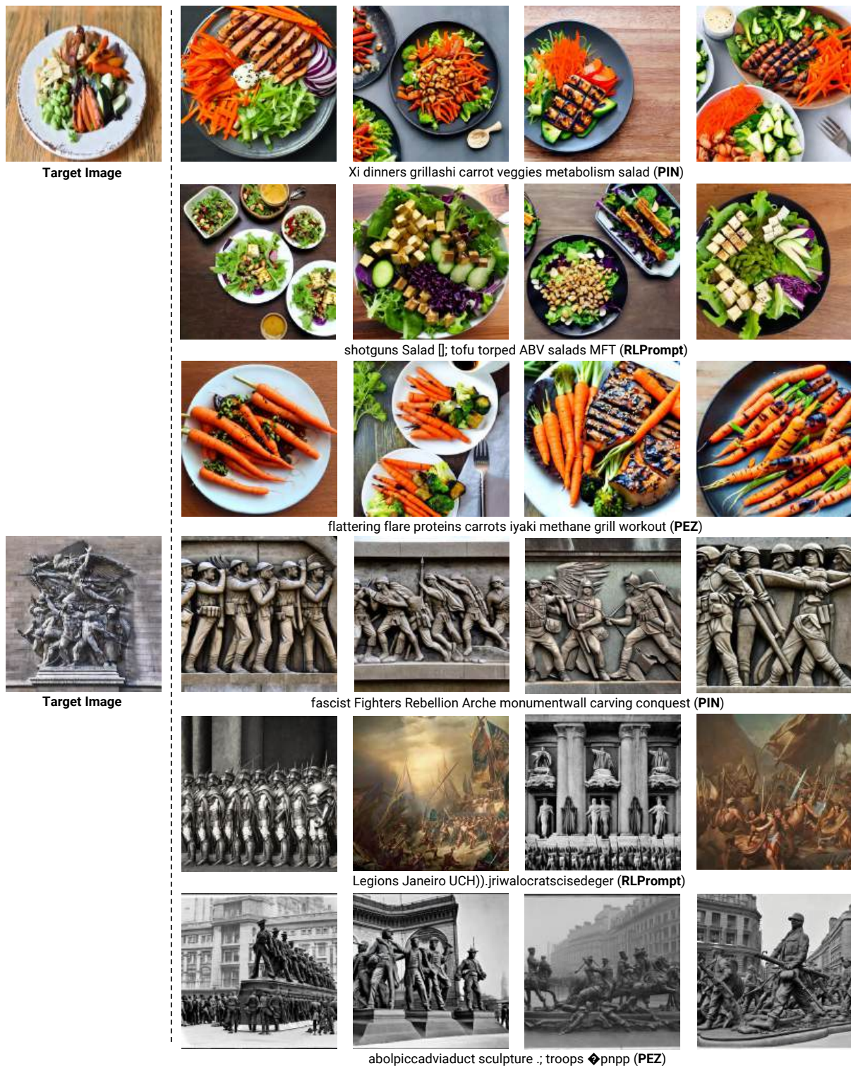
Figure 9: Generated images using learned hard prompts (bottom) through Stable Diffusion-v2 (Rombach et al., 2022) for a given target image (left).
