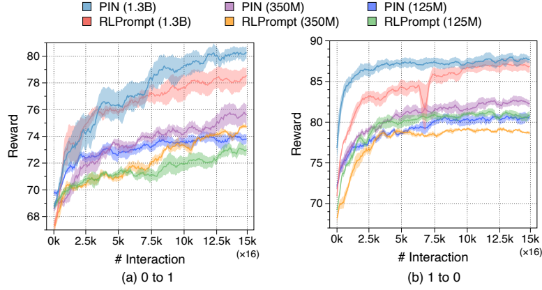
Figure 5: Training curve between our PIN method and RLPrompt over various task models (e.g. OPT-125M / 350M / 1.3B). For each dataset, specifically for sentiment style transfer including negative-to-positive (0 to 1) and positive-to-negative (1 to 0), 4 experiments were conducted with different seeds. The graph depicts the average reward on the validation set with standard error shading.
