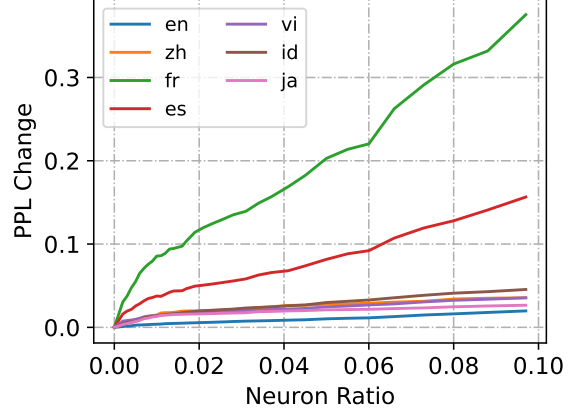
Figure 4: Change in PPL across different languages upon incremental number of language specific neurons when deactivating French neurons.
