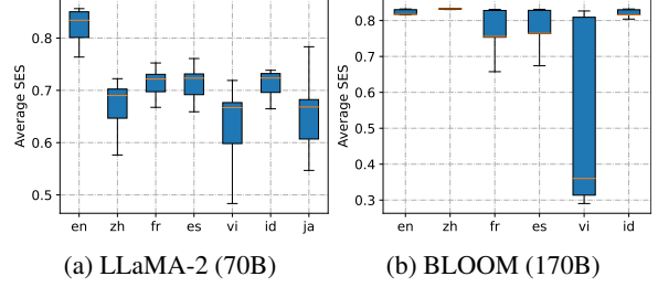
Figure 7: Dominance scores (mean SES) across layers when different languages serve as the target language.
