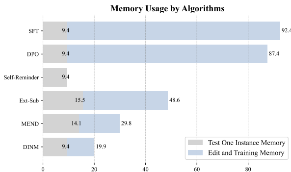
Figure 7: GPU VRAM consumption during training and editing for different approaches. We apply methods on Mistral-7B-v0.1 using 2 \times A800 .
