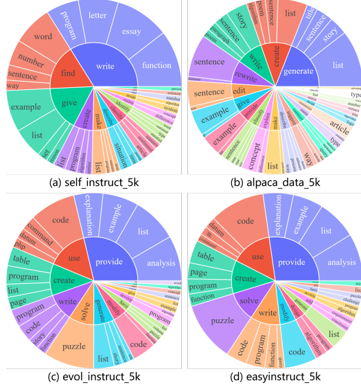
Figure 4: (Inner circle refers to the top 20 most prevalent root verbs and outer circle indicates their top 4 direct nouns in the generated instruction datasets considered in the experiments.
