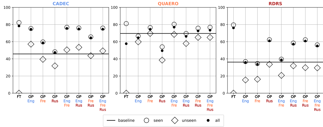
Figure 1: Performance of the FT and OP models on the three datasets, for each data partition ( seen , unseen and all ). The baseline is the zero-shot model in the target language.
