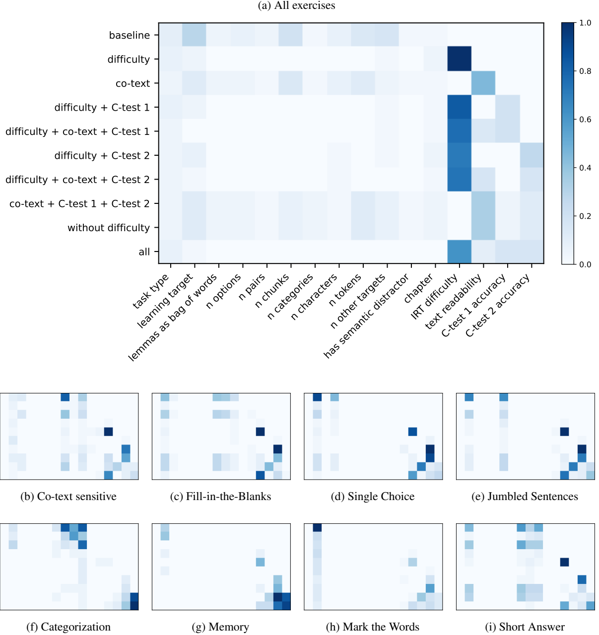
Figure 8: Feature importances
