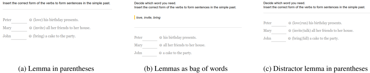
Figure 1: Codings of FiB exercises
