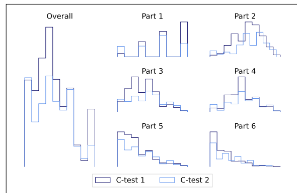
Figure 2: Distributions of C-test scores
