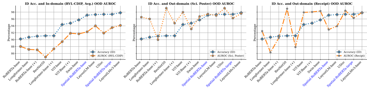
Figure 9: Correlation between ID accuracy and OOD detection performance. For most models, ID accuracy is positively correlated with OOD detection performance. Language models with spatial-aware adapters (highlighted in blue) achieve significantly higher ID accuracy and stronger OOD robustness (in AUROC) compared to language models without adapters. Here, (+) represents further pre-training on the IIT-CDIP dataset.
