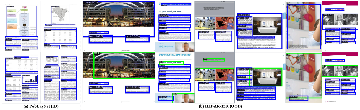
Figure 16: Visualization of detected objects on the OOD images (from IIIT-AR-13K) by a vanilla Faster-RCNN (top) and Faster-RCNN with VOS (bottom) is shown. Objects in blue boxes are detected and classified as one of the ID classes. The detected OOD objects (green) reduce false positives among detected objects. We also visualize detected objects on the ID images. There is a clear difference between PubLayNet and IIIT-AR-13K – entities and annotations of natural images rarely exist in PubLayNet.
