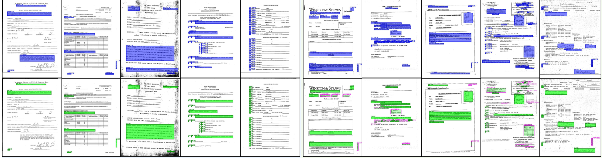
Figure 15: Visualization of detected OOD entities on the form images. The top part shows the entities in blue are entities annotated as other . The bottom part shows the detected OOD entities (green). We also show failure cases on the right part.
