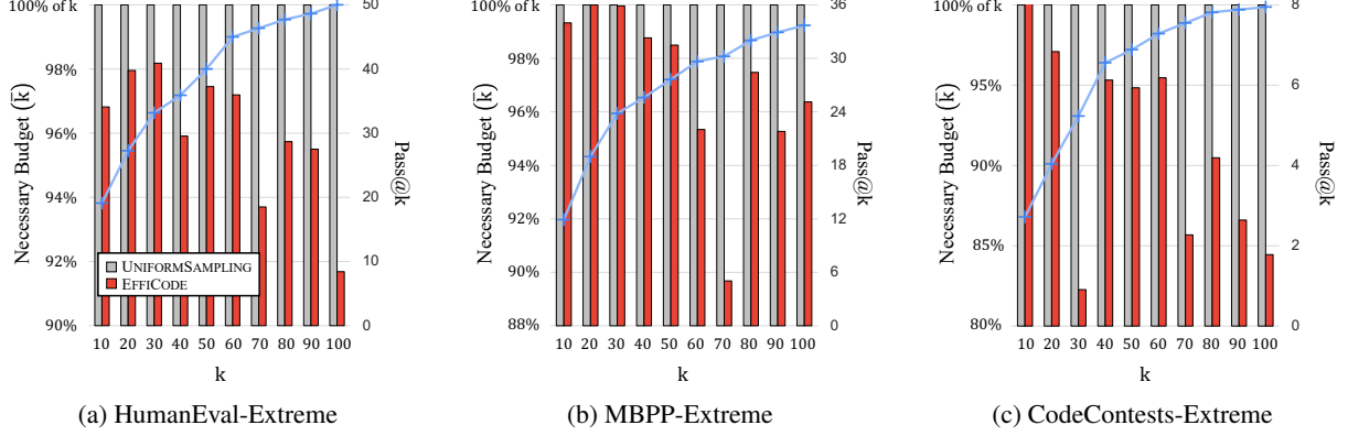
Figure 4: Results on various benchmarks with extreme settings. Bar charts, which belong to the left side of y-axis, denote the reduced amount of sampling budget to reach Pass@ k performance. Line charts belong to the right side of y-axis, indicating Pass@ k scores. Throughout the benchmarks, code samples were generated by GPT-3.5 with Self-planning.
