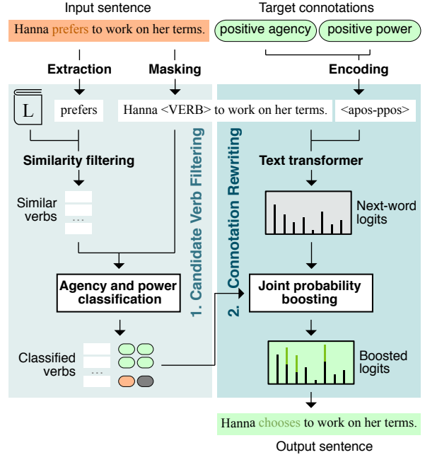
Figure 1: Proposed approach: After masking the verb in the input sentence, all similar verbs from a lexicon L are classified for agency and power in the sentence context. A transformer then rewrites the sentence. At each decoding step, the unnormalized token probabilities (logits) of verbs with target agency and power are increased.
