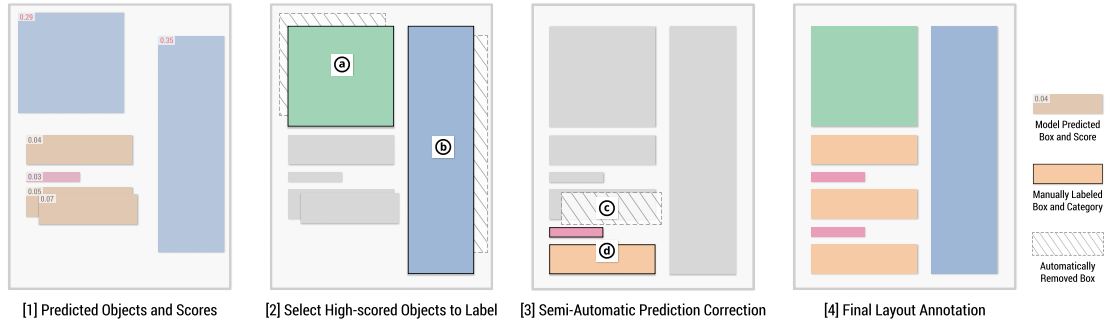
Figure 2: Illustration of the OLALA framework. [1] During labeling, for an input image, a trained model predicts the layout with various errors. An object scoring function f evaluates the informativeness for each object prediction. [2] OLALA selects the regions of top scores and sends them for manual labeling to correct the wrong object category (a) and bounding box (b). [3] A semi-automatic prediction correction algorithm is applied to rectify duplicated objects (c) and recover false-negatives (d) with minimal extra supervision. [4] After this process, the final annotation is obtained from labeling only a portion of the objects.
