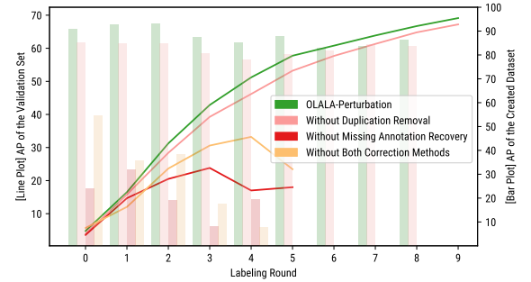
Figure 5: Influence of the prediction correction components on the model validation accuracy (line plot) and dataset accuracy (bar plot). Model performance suffers from removing the components, and dataset accuracy decreases accordingly. The Missing Annotation Recovery component, which corrects false negatives, is critical for model performance. Results shown are from experiments on PubLayNet.
