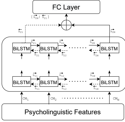
Figure 2: Structure diagram of BiLSTM emotion detection model trained on psycholinguistic features
