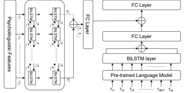
Figure 3: Structure diagram of hybrid emotion detection models
