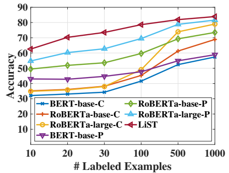
(a) MNLI
