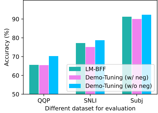
Figure 3: Ablation study on virtual demonstration optimization w/ Vs. w/o negative sampling. Demo-tuning (w/ neg): using conventional contrastive learning with negative samples to optimize virtual demonstration. Demo-tuning (w/o neg): Demo-tuning using our simplified optimization method without negative samples.
