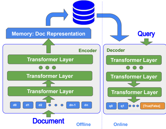
Figure 1: Overview of the proposed ED2LM.
