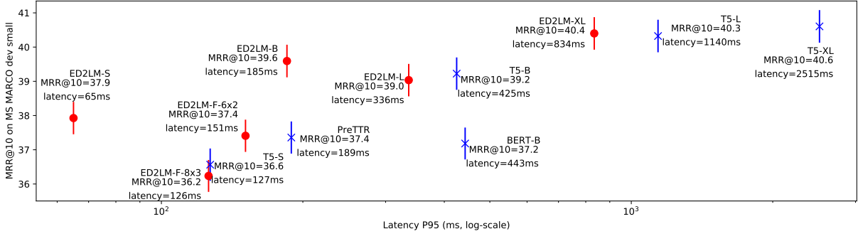
Figure 2: MRR@10 on MS MARCO dev small (6980 test queries) after re-ranking top-1K documents from docT5query (Nogueira et al., 2019a) vs. latency. The x-axis is the latency (95 percentile out of 500 calls); y-axis is the MRR@10 score. The point (ED2LM models) and the cross (baseline models) are the mean MRR@10 and the bar indicates the 95% confidence interval.
