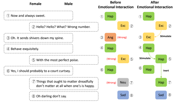
Figure 3: A case study based on IEMOCAP dataset.
