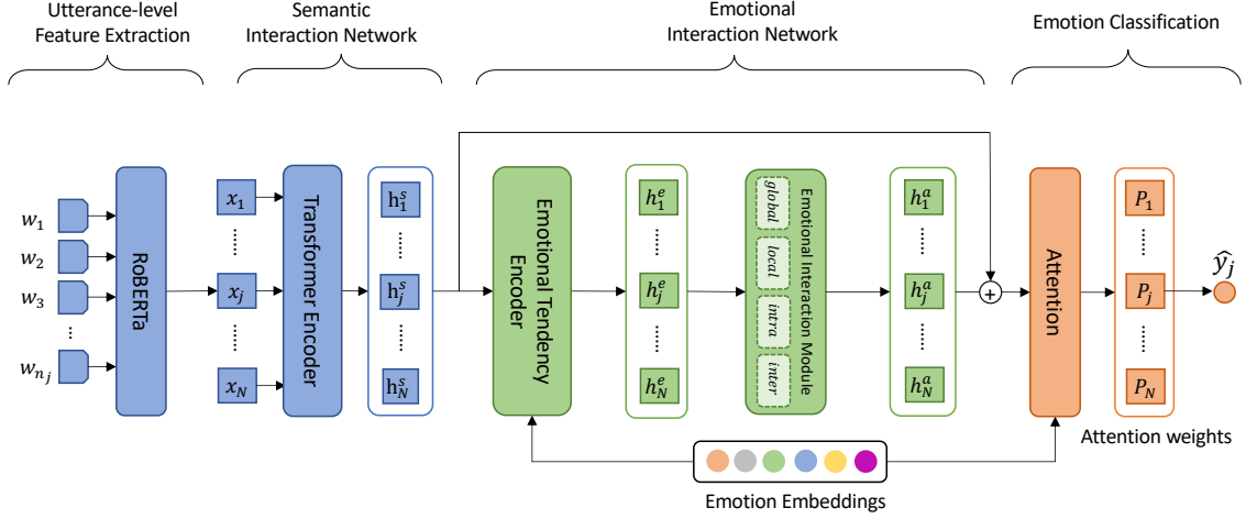
Figure 2: Framework illustration of DialogueEIN, which consists of four key components: Utterance-level Feature Extraction, Semantic Interaction Network, Emotional Interaction Network, Emotion Classification.
