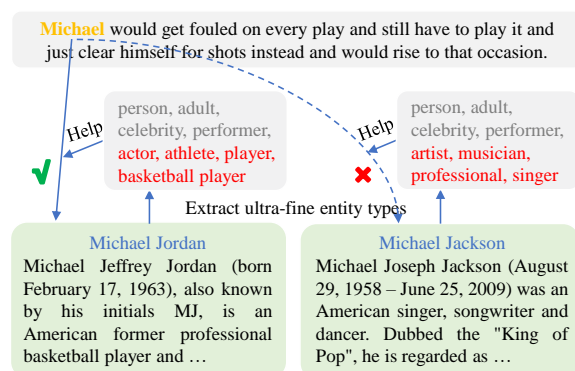
Figure 1: Examples of entity linking with general ultra-fine-grained entity type information. Different ultra-fine-grained types of the two entities are denoted in red.
