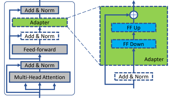
Figure 2: Left: location of an adapter (green box) inside a layer of the pretrained transformer. Gray boxes represent the original components of a transformer layer. Right: the network architecture of an adapter.
