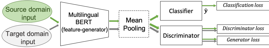
(a) Keung et al. (2019) . The source features and target features are only input to the discriminator to calculate the discriminator loss and the generator loss. For the classification loss, mean pooling is not applied to NER.
