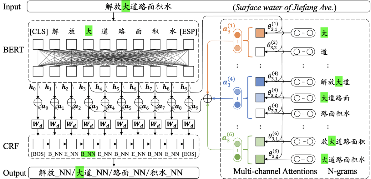
Figure 2: The overall architecture of our character-based model for the joint CWS and POS tagging with an example input and output. On the left is the backbone model following the sequence labeling paradigm; on the right is the multi-channel attention module with n-grams categorized by their length. Different attention channels for n-grams associated with “大” ( big ) are highlighted with distinct colors.
