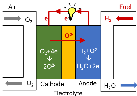
Figure 2: Solid Oxide Fuel Cell schema.
