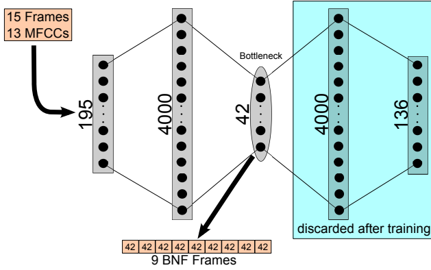
Figure 1: The MLP architecture (4kx4k) that performed best in our experiments: A 15 frame context window, with 13 MFCCs each, was used as the input feature; the 136 node target layer (one node per sub-phone) and the 4k 3rd hidden layer were discarded after the MLP was trained. A 9 frame context window of the MLP output at the 42 node bottleneck layer is then used as the new 378 dim BNF feature.
