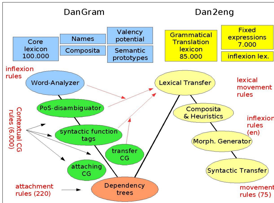
Figure 1: Dan2Eng system architecture
